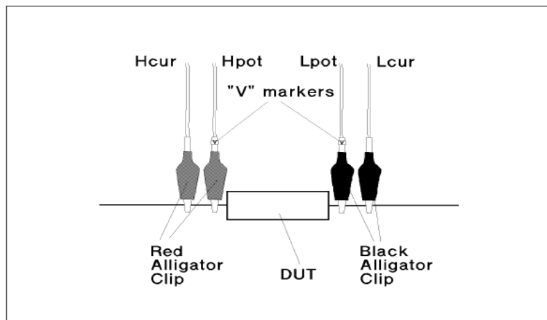
Connecting the DUT to the 16089D
